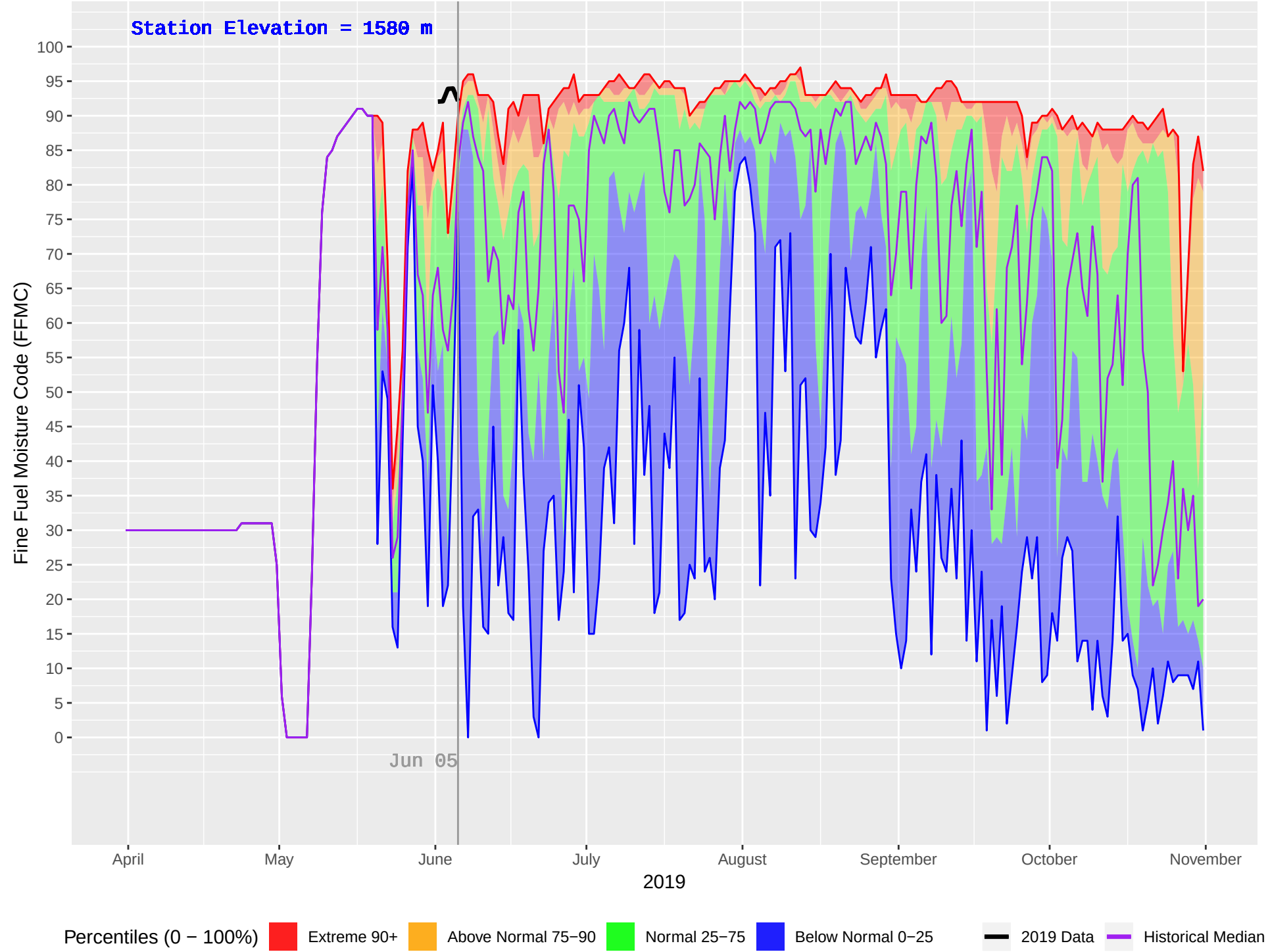
RORY CREEK (1092) : Historical (2010–2018) and Current (2019) Daily Fine Fuel Moisture Code (FFMC)
