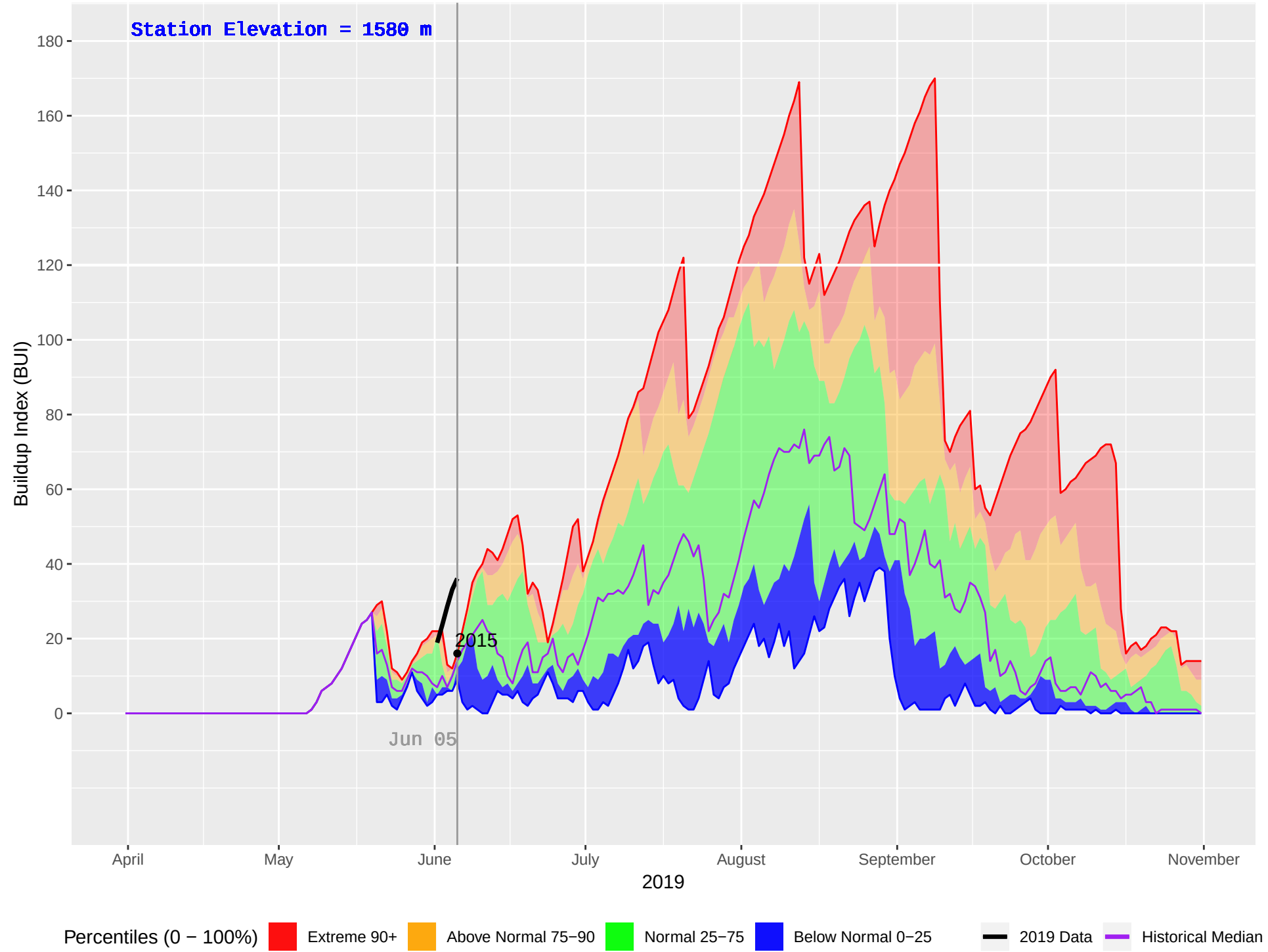
RORY CREEK (1092) : Historical (2010–2018), Current (2019) Daily Buildup Index (BUI)
