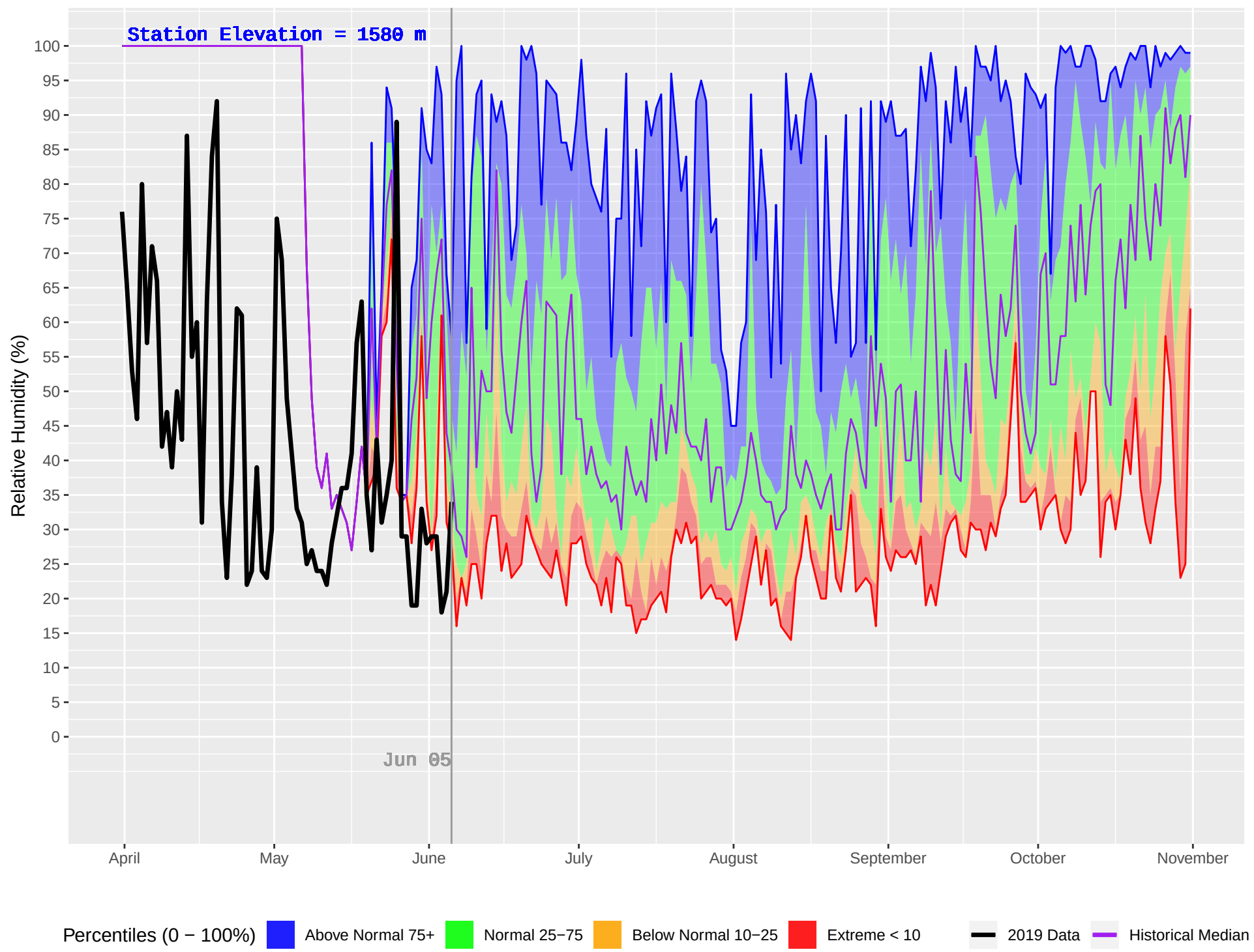
RORY CREEK (1092) : Historical (2010–2018) and Current (2019) Daily Relative Humidity
