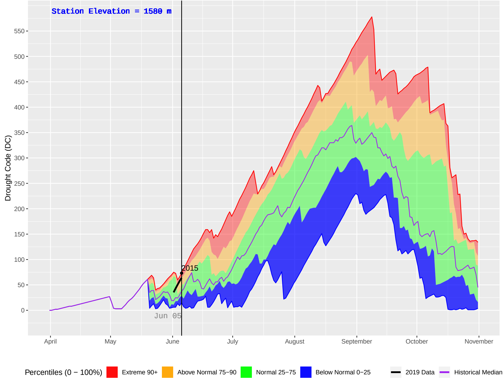
RORY CREEK (1092) : Historical (2010–2018) and Current (2019) Daily Drought Code (DC)
