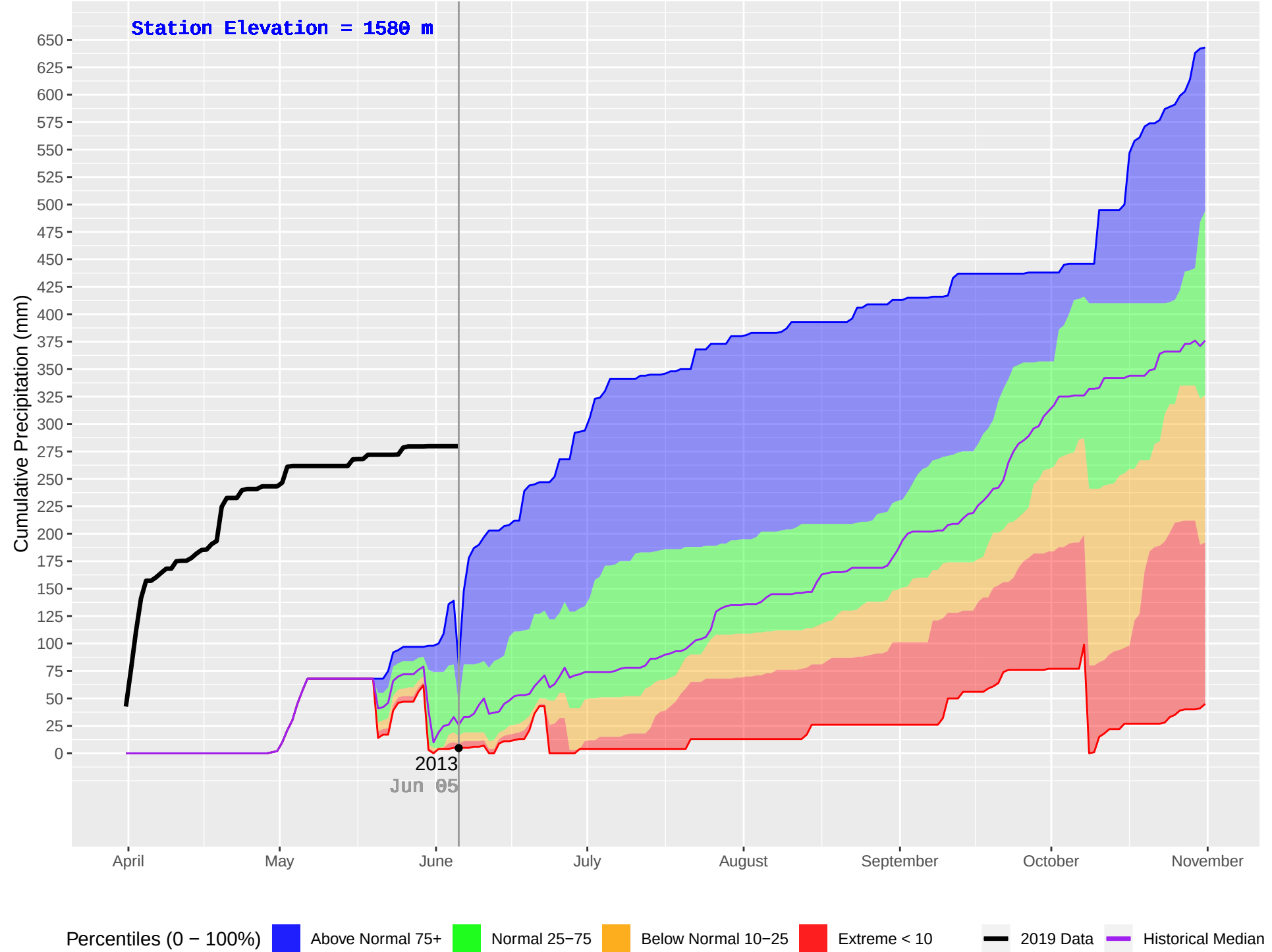
RORY CREEK (1092) : Historical (2010–2018), Current (2019) Daily Cumulative Precipitation
