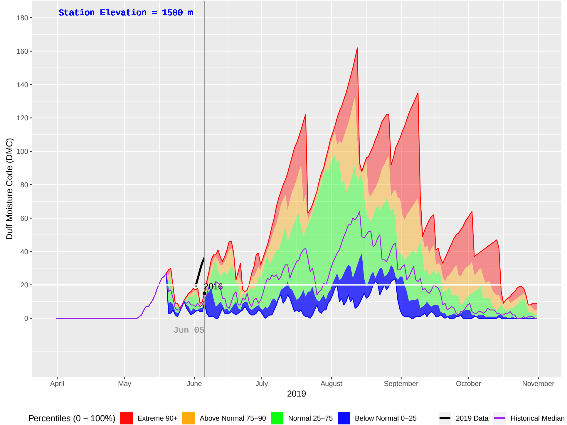
RORY CREEK (1092) : Historical (2010–2018), Current (2019) Daily Duff Moisture Code (DMC)
